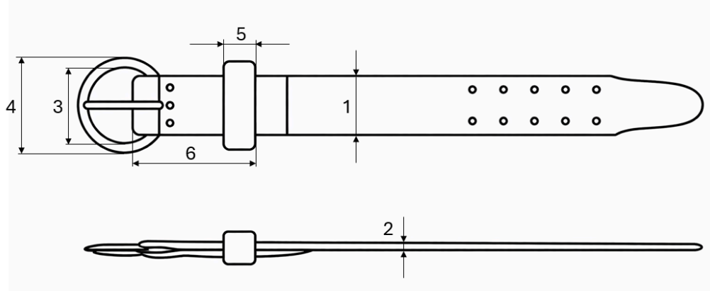
Fig. 3: Dimensions of the squat belt
